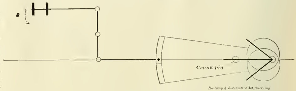
OUTSIDE ADMISSION—INDIRECT.
